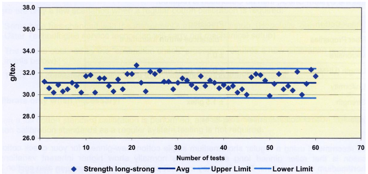
Figure: Control chart [Uster Technologies]
